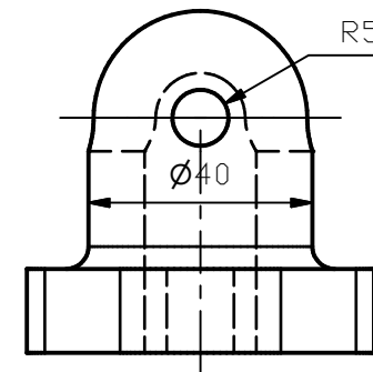
LEFT VIEW
